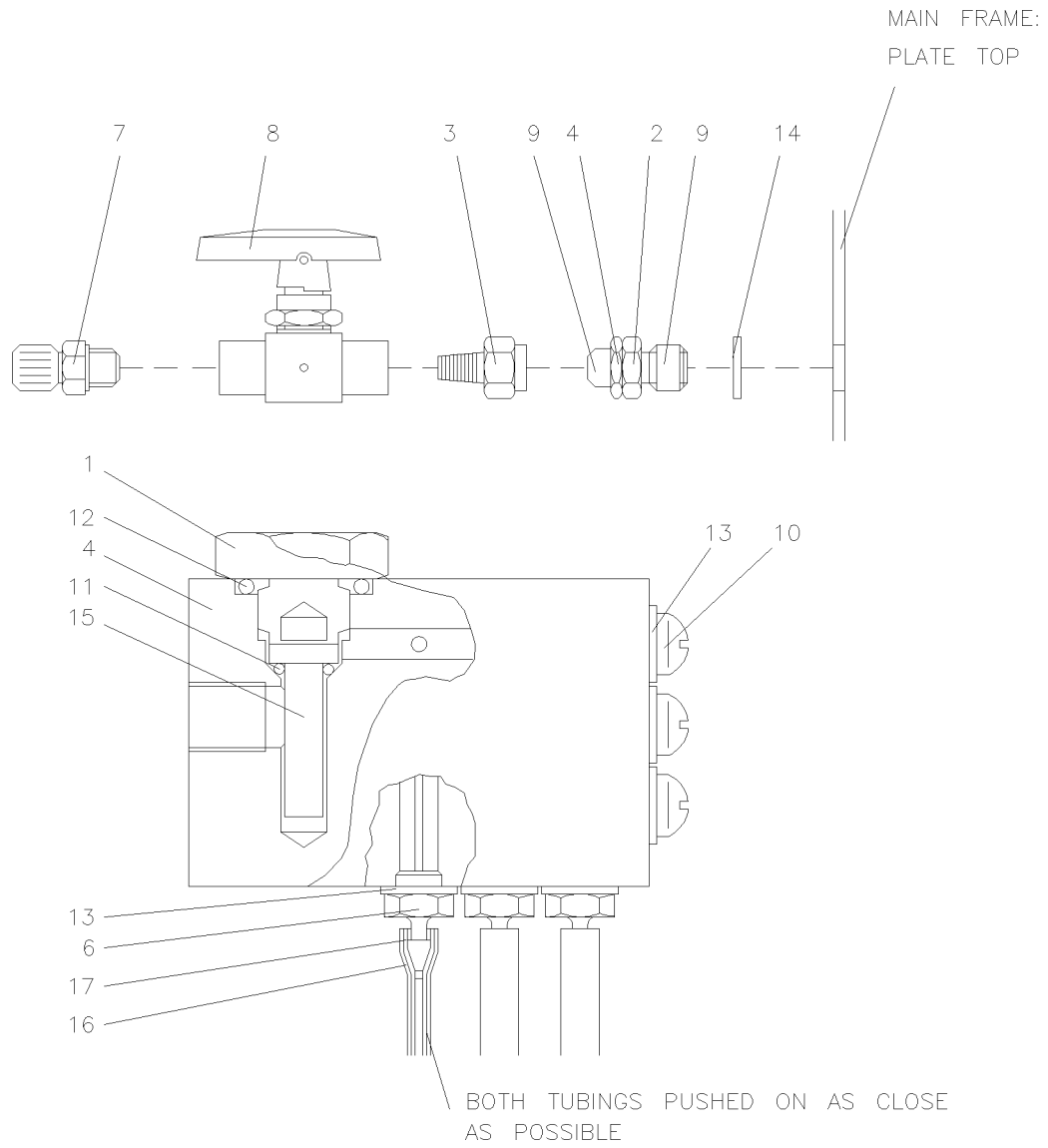
Figure 20-1. Helium Inlet
